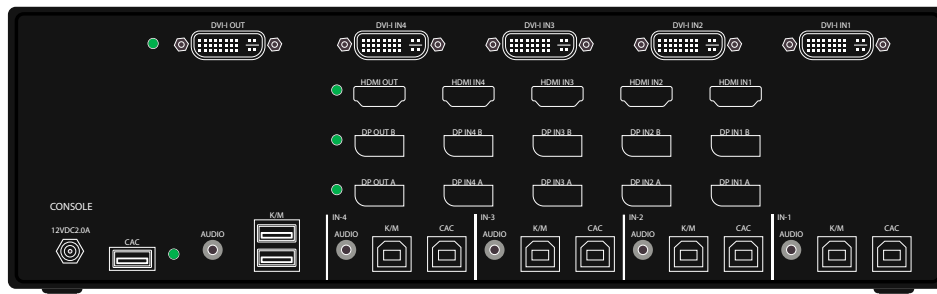
Figure 4-2: SA-DPH-4Q-P Rear panel
