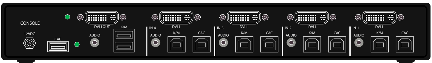
Figure 4-2: SA-DVN-4S-P Rear panel
