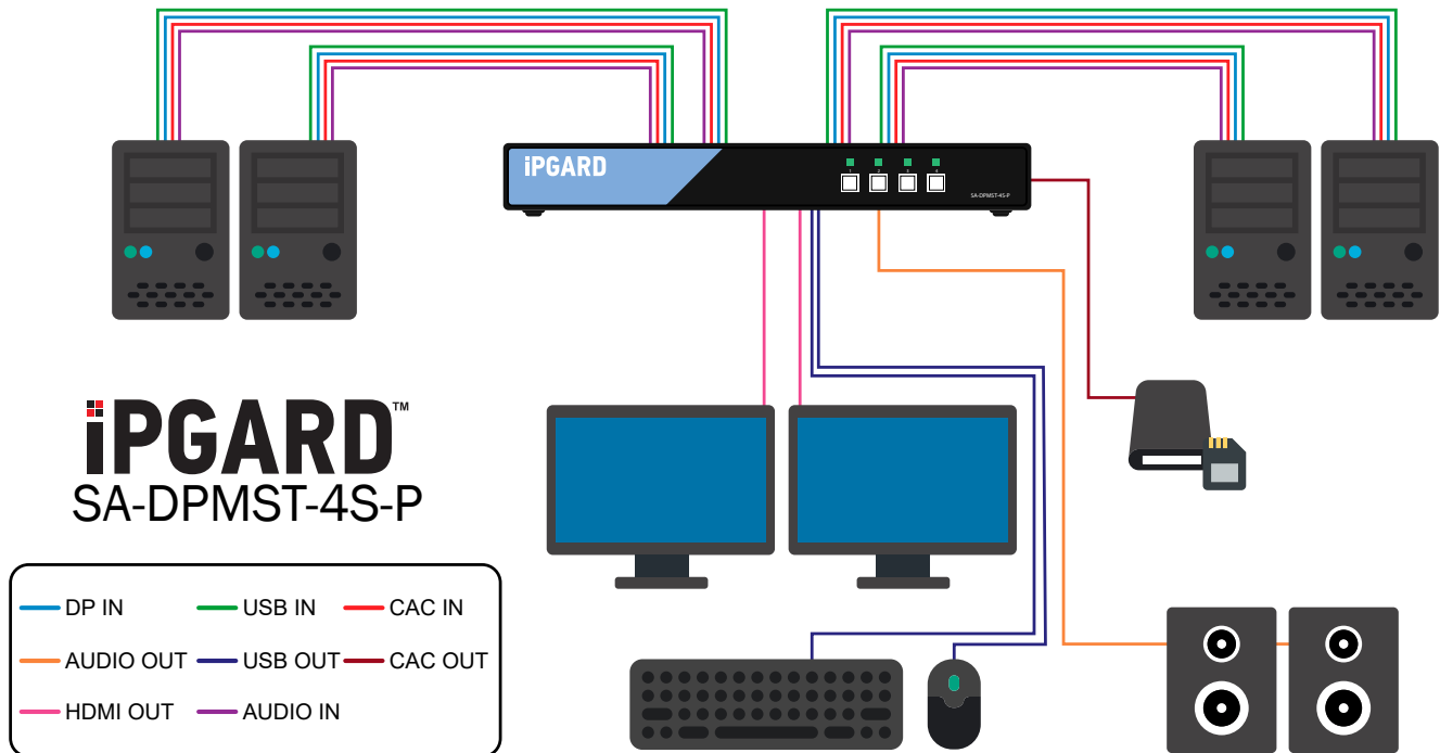
Figure 6-1: SA-DPMST-4S-P
