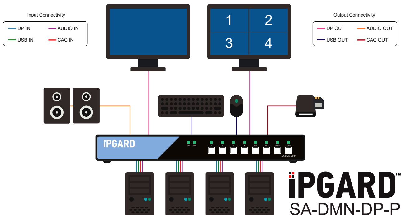
Figure 6-1: SA-DMN-DP-P
