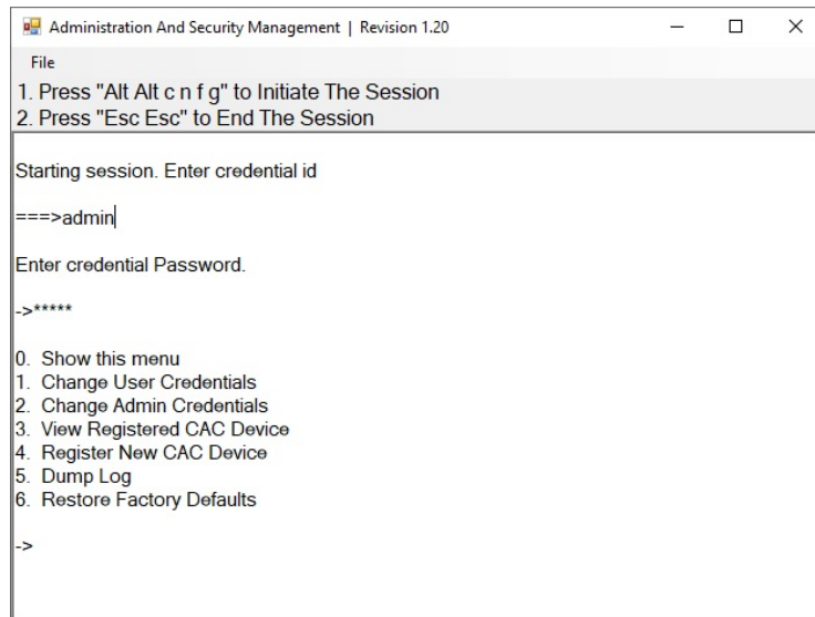
Figure 7: Administrator Log-in
