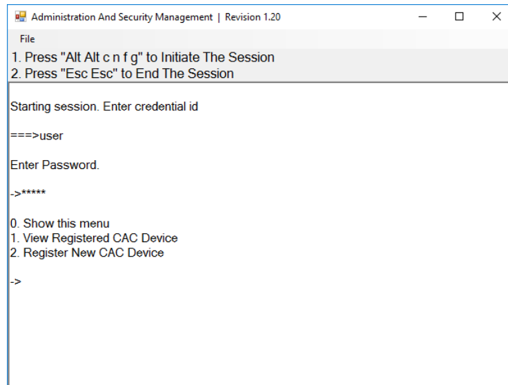
Figure 3: User Log-in
