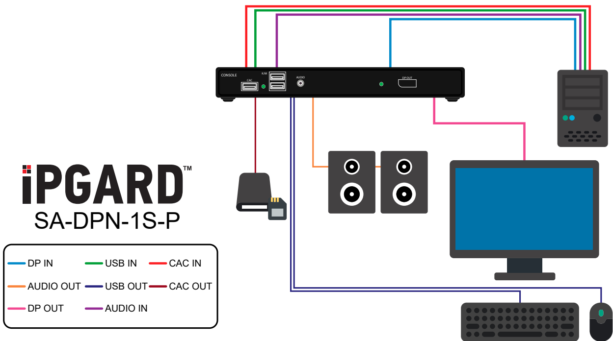
Figure 6-1: SA-DPN-1S-P
