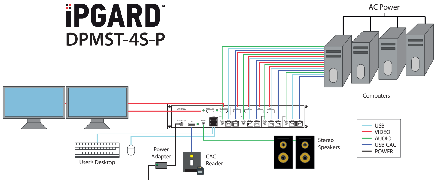
Figure 6-1: DPMST-4S-P
