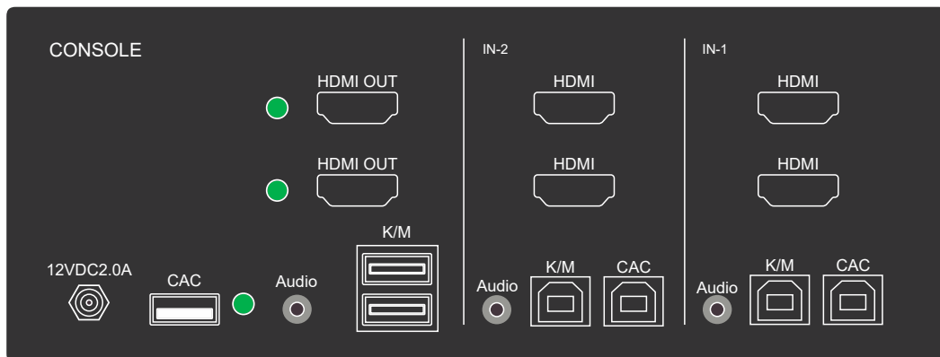
SUHN-2D-P Back
