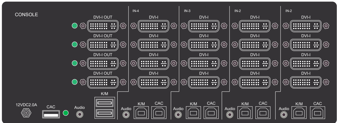
SDVN-4Q-P Back
