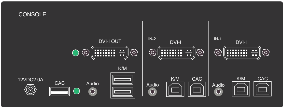
SDVN-2S-P Back
