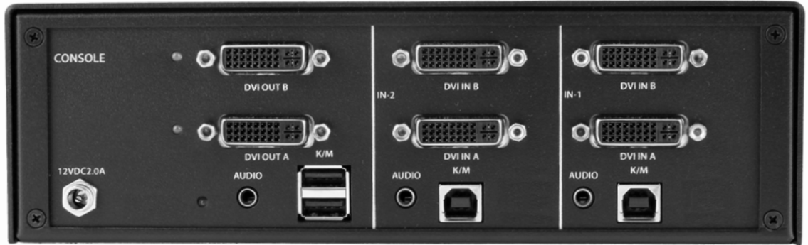
SDVN-2D Back
