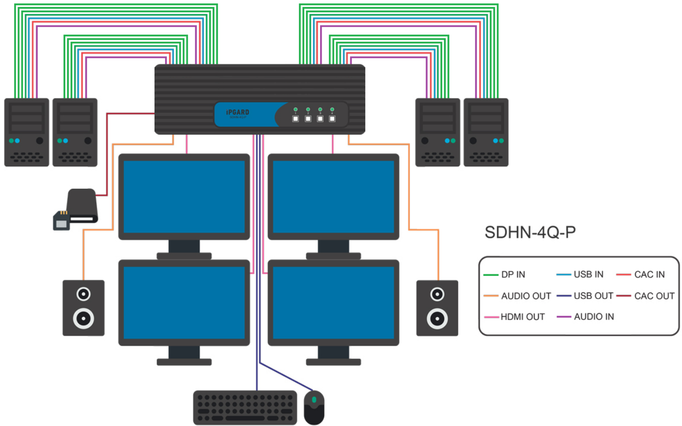
Figure 8-1 SDHN-4Q-P Shown
