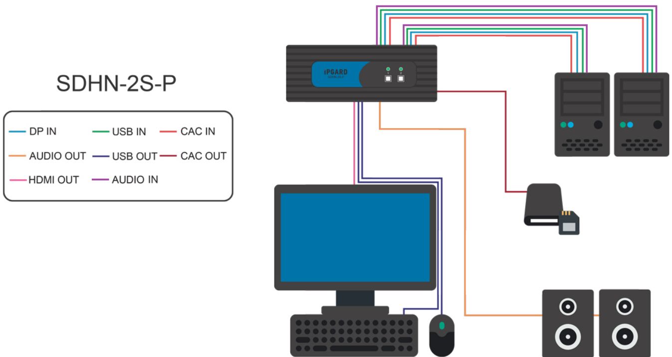
Figure 8-2 SDHN-2S-P Shown
