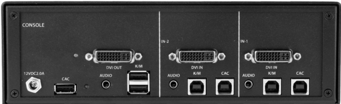
SDVN-2S-P Back
